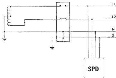
FIG. 1: Split Phase, 3-Wire
